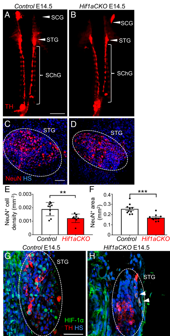
Fig. 8. The growth and maturation of secondary sympathetic ganglia are impaired in E14.5 Hif1a CKO embryos. (A and B) Whole-mount TH immunostaining was performed to detect the secondary chain of sympathetic ganglia, which are smaller in Hif1a CKO mice compared with control littermates. Arrowheads indicate the superior cervical (SCG) and stellate (STG) ganglia; bracket indicates the thoracic chain of sympathetic ganglia (SchG). (Scale bar: 1,000 \mu m.) (C and D) Immunostaining for NeuN (a marker for differentiated neurons; red) shows reduced neuronal density in the STG of Hif1a CKO compared with control embryos ( n = 5 embryos per genotype and 2 ganglia per embryo). **P < 0.01 , Student's t test. (Scale bar: 50 \mu m.) (E and F) Morphometry of sympathetic ganglia (the STG and three upper ganglia of the thoracic sympathetic chain) by whole-mount NeuN immunostaining of the spinal cord ( n = 5 embryos per genotype, left and right sympathetic chain ganglia per embryo). ***P < 0.0005 , Student's t test. (G and H) Coronal sections of embryos immunolabeled with anti-TH (red) and anti-HIF-1 \alpha (green) show a smaller STG area (dotted oval) and lower HIF-1 \alpha expression in Hif1a CKO embryos. Strong HIF-1 \alpha expression was detected in nuclei of TH + neurons in control embryos (G) but only in the cytoplasm of a few TH + neurons in Hif1a CKO embryos (H, arrowheads). (Scale bar: 50 \mu m.) All numerical data are presented as mean \pm SEM.
