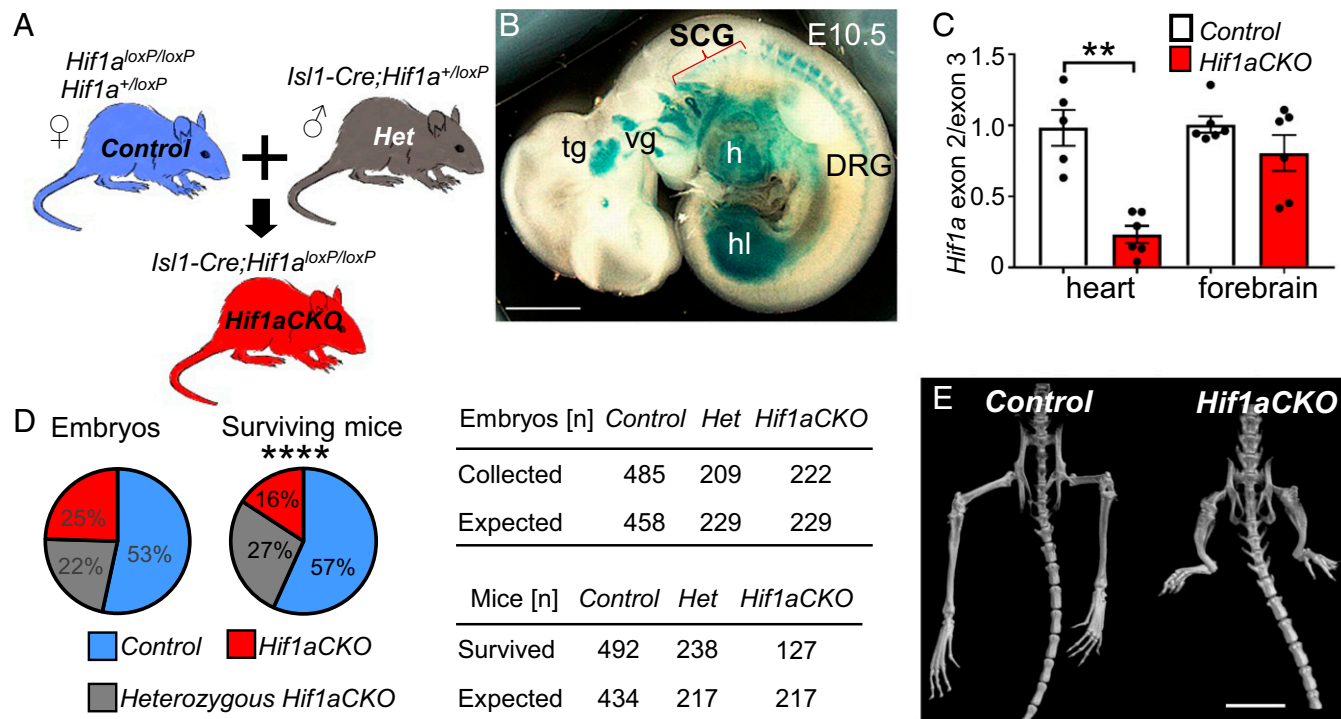
Fig. 1. Decreased neonatal survival and hindlimb malformations in Hif1aCKO mice. (A) The Isl1-Cre transgene was transmitted paternally to eliminate any potential influence of maternal HIF-1 \alpha haploinsufficiency on the developing embryos. (B) Whole-mount X-gal staining of E10.5 Isl1-Cre;Rosa 26R embryos revealed \beta -galactosidase expression in the dorsal root ganglia (DRG) and sympathetic cervical ganglia (SCG), trigeminal ganglion (tg), vestibular ganglion (vg), heart (h), and hindlimb (hl). (Scale bar: 100 \mu m.) (C) qPCR analysis of exon 2 (normalized to exon 3) sequences in genomic DNA isolated from heart and forebrain of Hif1aCKO and control embryos at E10.5. The data are presented as mean \pm SEM ( n = 6 embryos per group). **P < 0.01 , Student's t test. (D, Left) The genotype distribution of embryos and surviving mice. (D, Right) Observed distribution of genotypes of embryos collected between E7.5 and E17.5 according to the expected Mendelian ratio (Top). In contrast, the observed genotype distribution of surviving mice at 3 wk after birth shows a decreased number of Hif1aCKO mice (Bottom). ****P < 0.0001 , \chi^2 test. (E) Micro-CT scan shows hindlimb malformations with reduced tibia, femur, and pelvis lengths in adult Hif1aCKO mice. (Scale bar: 10 mm.)
